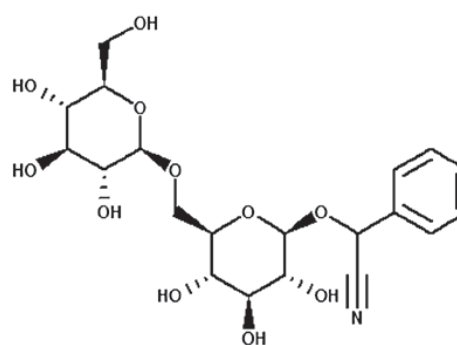
Figure 1. Chemical structure of amygdalin.
